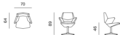
CONFERENCE CHAIR dimensions 70 x 64 x 89 cm
