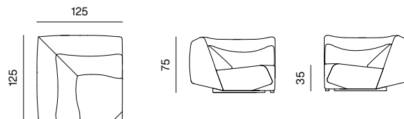
CORNER M LOW dimensions 125 × 125 × 75 cm
