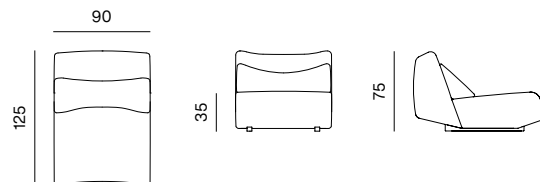
SEAT M + BACKREST LOW dimensions 90 × 125 × 75 cm
