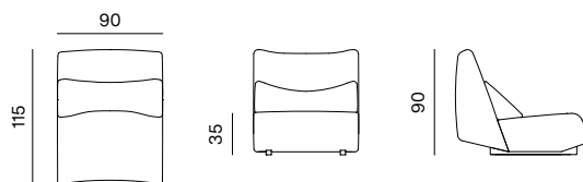
SEAT S + BACKREST HIGH dimensions 90 × 115 × 90 cm
