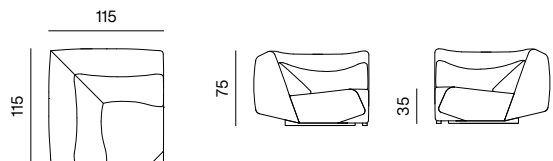
CORNER S LOW dimensions 115 × 115 × 75 cm
