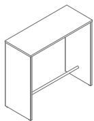
PSW52 1200 / 500 / 1100 42.3 kg
