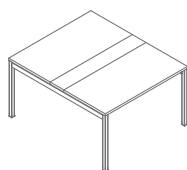
SY22 1200 / 1410 / 740 61.1 kg
