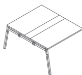
SW42L 1200 / 1410 / 740 51.9 kg
